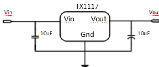
Application circuit of TX1117 fixed version
