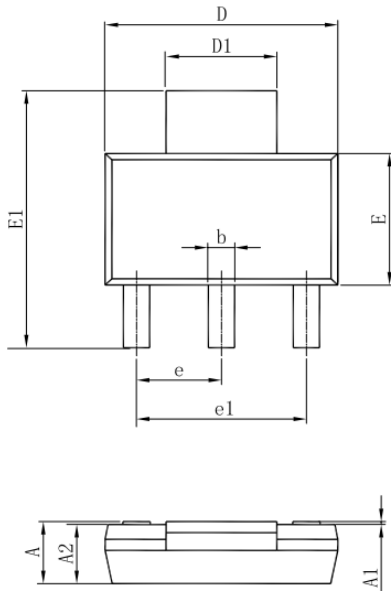
SOT-223 PACKAGE OUTLINE DIMENSIONS
