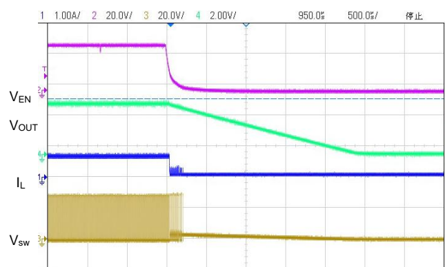
(18) Enable Shutdown(VIN=30.0V,VOUT=3.3V,IOUT=0.6A)
