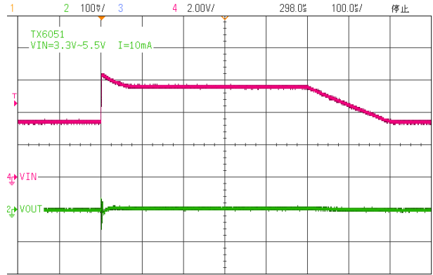
(14) Input Transient Response (VIN=3.3V-5.5V)
