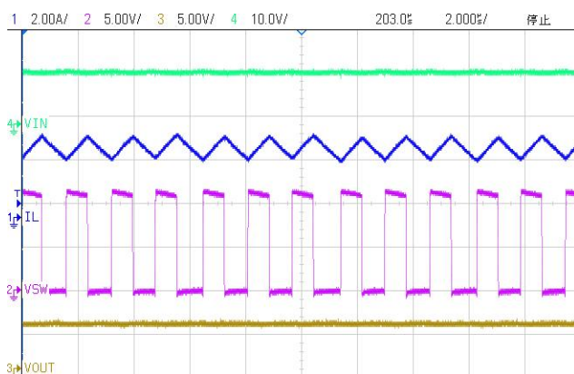
(23) Steady State (VIN=12.0V, VOUT=5.0V, IOUT=3A)
