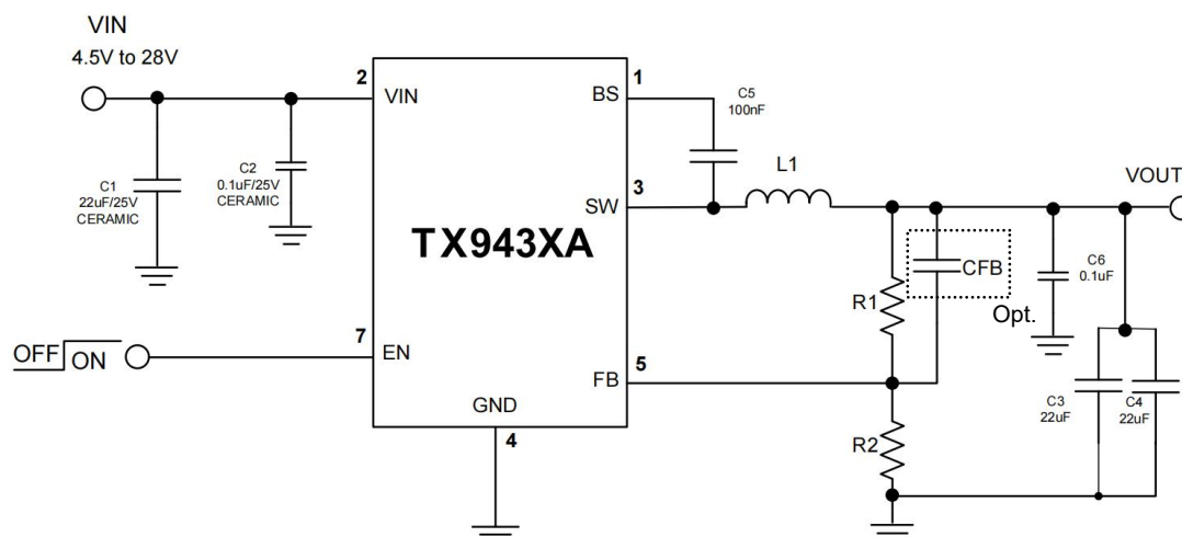
图 1. Basic Application Circuit
