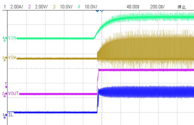
(19) Power Ramp Up (VIN=15.0V, VOUT=3.3V, IOUT=3A)
