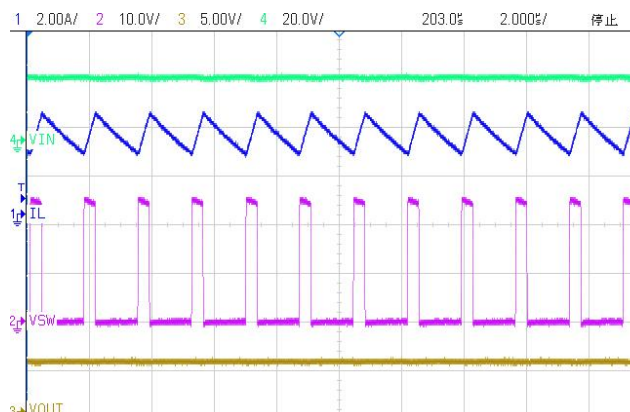
(24) Steady State (VIN=26.0V, VOUT=5.0V, IOUT=3A)
