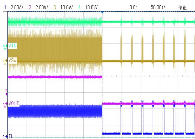
(23) Steady State (VIN=12.0V, VOUT=5.0V, IOUT=3A)
