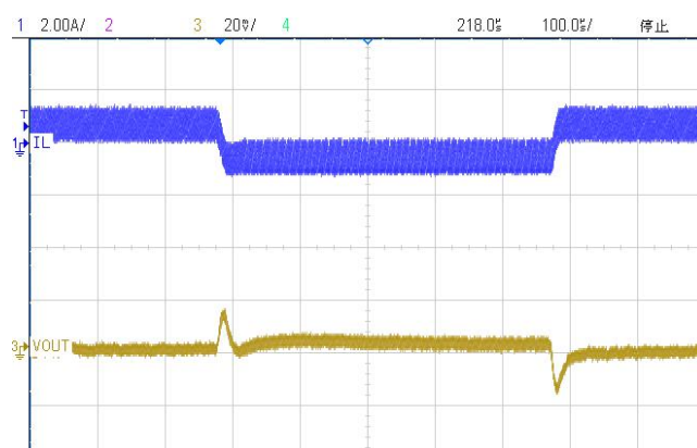
(16) Load Transient(VIN=15.0V,VOUT=5.0V,IOUT=0.5→1.8A)
