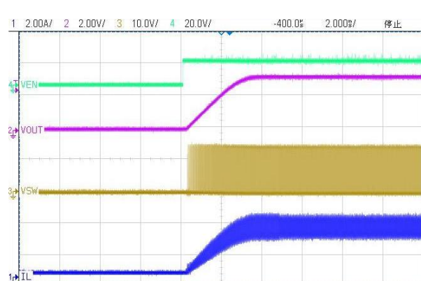
(17) Enable Start Up (VIN=15.0V,VOUT=3.3V,IOUT=3A)
