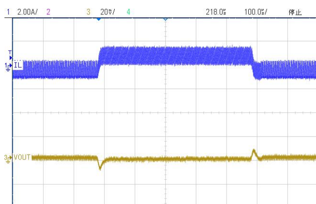
(15) Load Transient (VIN=15.0V,VOUT=3.3V,IOUT=0.5→1.8A)
