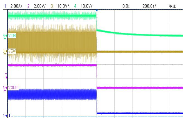
(20) Power Ramp Down (VIN=15.0V, VOUT=3.3V, IOUT=3A)
