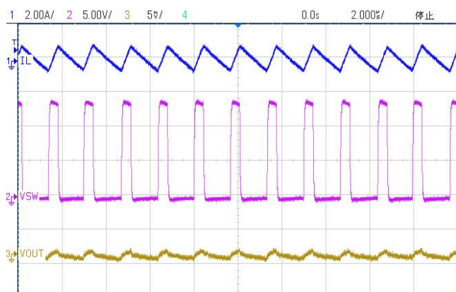
(13) Output Ripple (VIN=15.0V,VOUT=3.3V,IOUT=3A)
