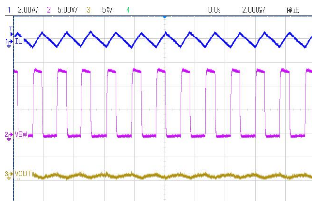
(14) Output Ripple (VIN=15.0V,VOUT=5.0V,IOUT=3A)
