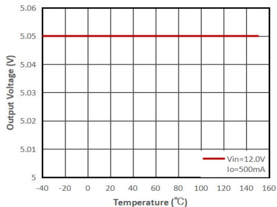
(12) Output Voltage VS Temperature ( V_{OUT}=5.0V )
