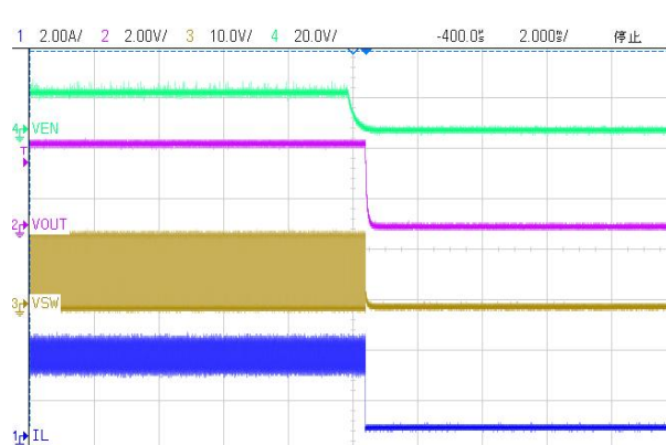
(18) Enable Shutdown(VIN=15.0V,VOUT=3.3V,IOUT=3A)
