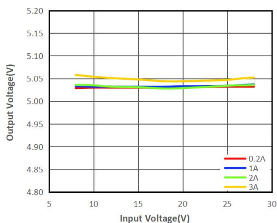
(6) Output Voltage VS Input Voltage ( V_{OUT} = 5.0V )
