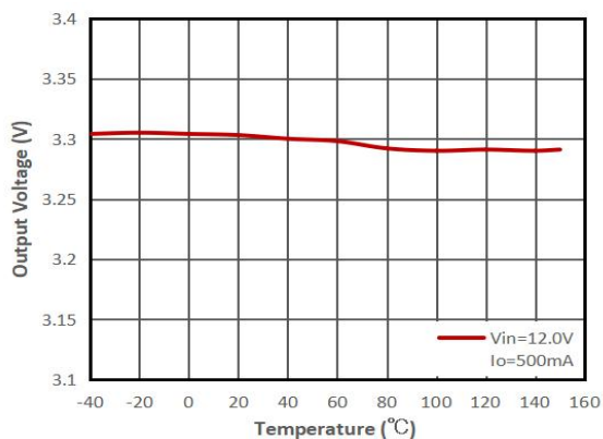
(11) Output Voltage VS Temperature ( V_{OUT}=3.3V )
