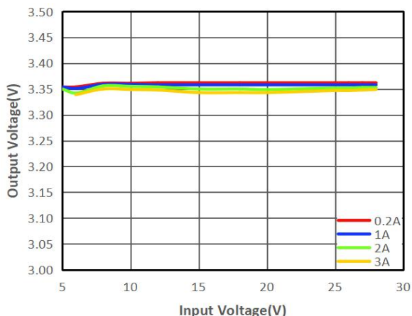
(5) Output Voltage VS Input Voltage ( V_{OUT} = 3.3V )
