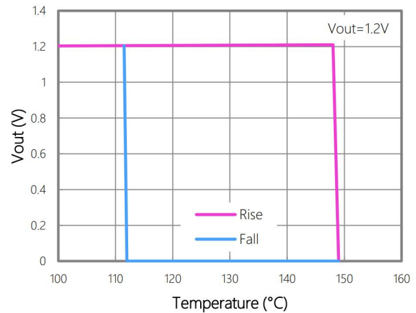
OTP Hystersis
