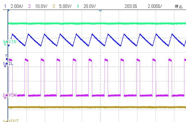
(24) Steady State (VIN=26.0V, VOUT=5.0V, IOUT=3A)
