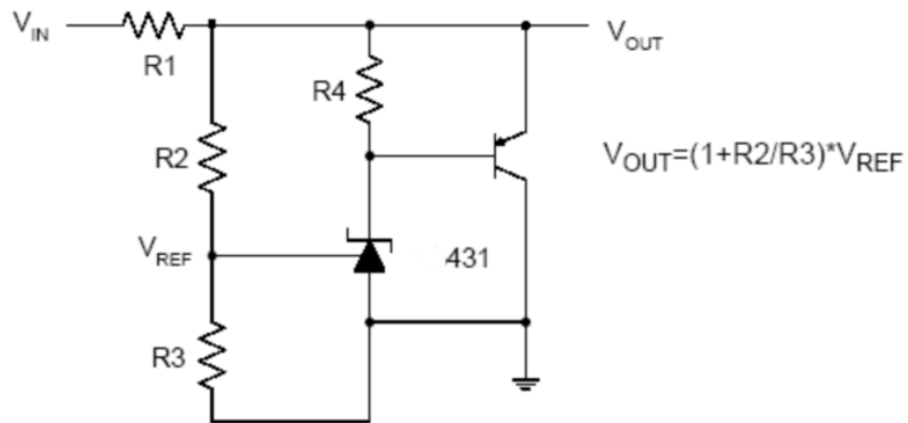
Shunt Regulator
