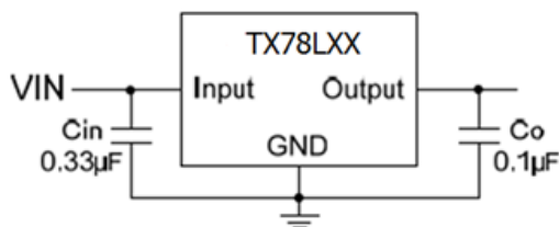
Fig.1 Typical Application
