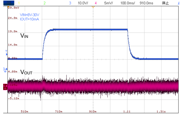
(16) Input Transient Response ( V_{IN}=8V-30V )
